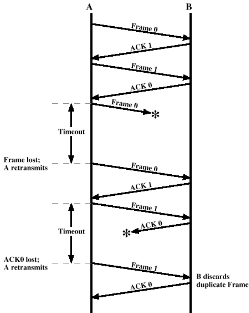
Gambar 5.10. Stop-and-wait ARQ.
